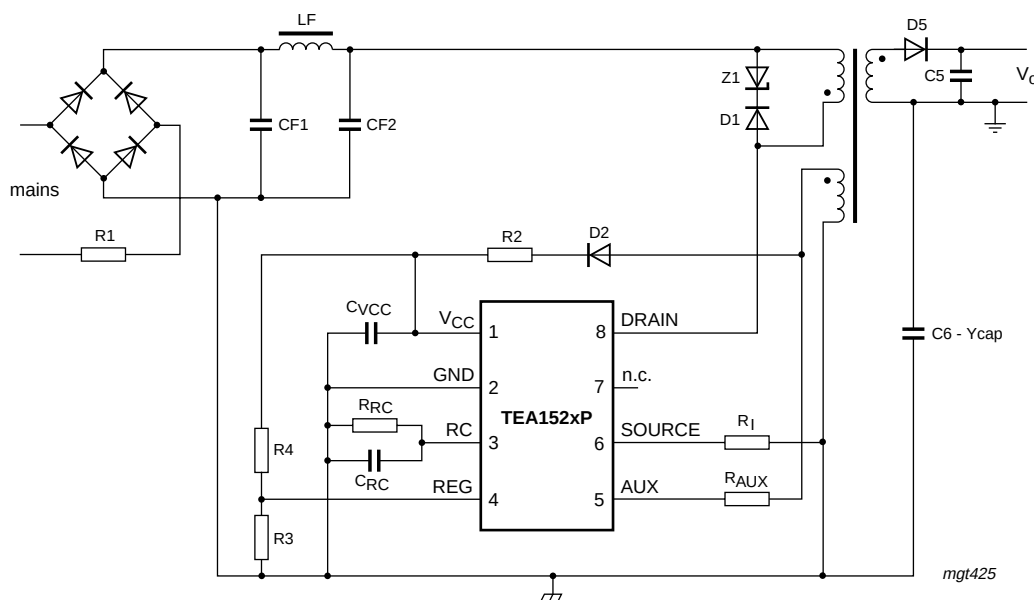
Fig 6. Primary sensed application; configuration for TEA152xP
